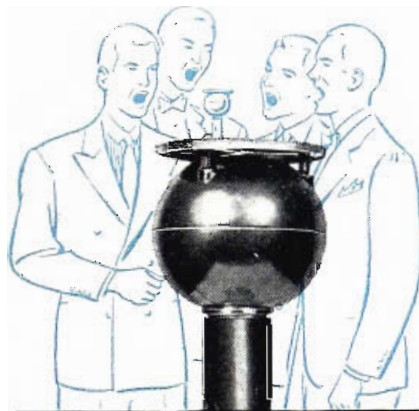
1935: The first non-directional mike—the famous Western Electric B-Ball, designed by Bell Laboratories. Small, spherical, it provided top quality single mike pick-up of speech or music from every direction.
